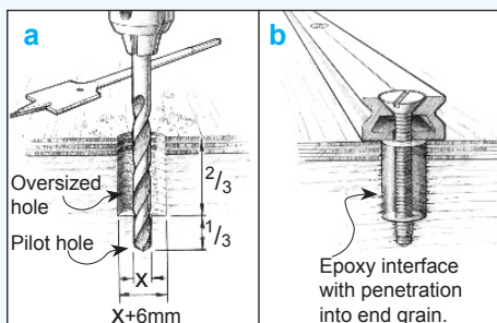
Figure 16 Drill oversized holes to increase the exposed substrate area and the amount of epoxy around the fastener.
